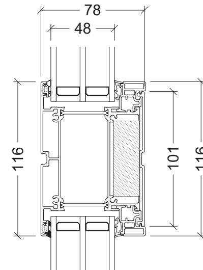
116mm glazing bar
