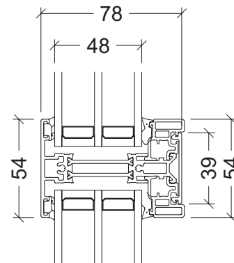
54mm glazing bar
