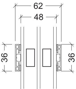
36mm energy glazing bar
