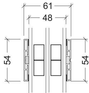
54mm energy glazing bar
